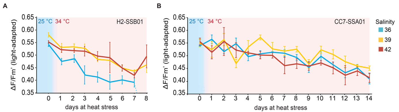
Fig. 3. Effect of different salinities on photosynthetic efficiency during heat stress in the coral model Aiptasia . Day 0 marks the end of a 10-day acclimation phase at 25°C, after which the temperature was increased to 34°C. Color key indicates salinity: blue (36), yellow (39), red (42). (A) Aiptasia H2 associated with Symbiodinium SSB01 showed significantly reduced impairment of photosynthetic efficiencies at increased salinities under heat stress. The heat stress treatment was concluded on day 8 due to substantial bleaching and the fluorescent signal being too low to be measured by Pulse Amplitude Modulated (PAM) fluorometry at a salinity of 36. (B) Photosynthetic efficiency of Aiptasia CC7 associated with Symbiodinium SSA01 was significantly less impaired at a salinity of 39 in comparison to the salinities of 36 and 42. Heat stress continued until day 14, when the photosynthetic efficiency for one of the measurements dropped below 0.4. Data are shown as means \pm s.e.
