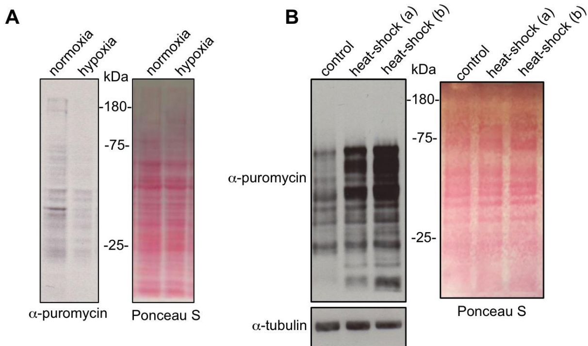
Fig. 4. Regulation of larval protein synthesis by hypoxia and heat stress. (A) Third instar larvae were either maintained in room air (normoxia) or exposed to 5% O 2 (hypoxia) for four hours. Larvae were then inverted and incubated in Schneider's media + puromycin (5 \mu g/ml) for 40 mins. Equal amounts of whole larval protein extracts were then analyzed by western blotting. Left, western blot with anti-puromycin antibody. Right, Ponceau S staining showing total protein levels. (B) Third instar were either maintained at 25 ^{\circ} C (control) or exposed to a one hour 37 ^{\circ} C heat-shock. Larvae were then inverted and incubated in Schneider's media + puromycin (5 \mu g/ml) for 40 mins. For the heat-shock samples the puromycin incubation was carried out either at room temperature (a) or at 37 ^{\circ} C (b). Equal amounts of whole larval protein extracts were then analyzed by western blotting Left, western blot with anti-puromycin antibody or anti-tubulin antibody. Right, Ponceau S staining showing total protein levels. All experiments in Fig 4 were carried out using w 1118 larvae.
