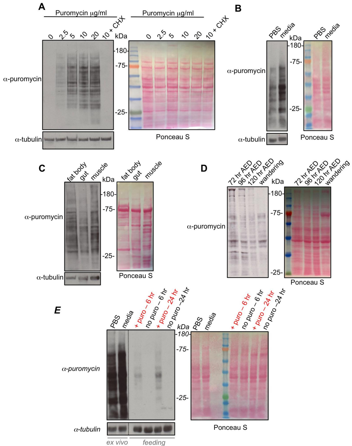
Fig. 1. Puromycin-labelling to measure protein synthesis during larval development.
