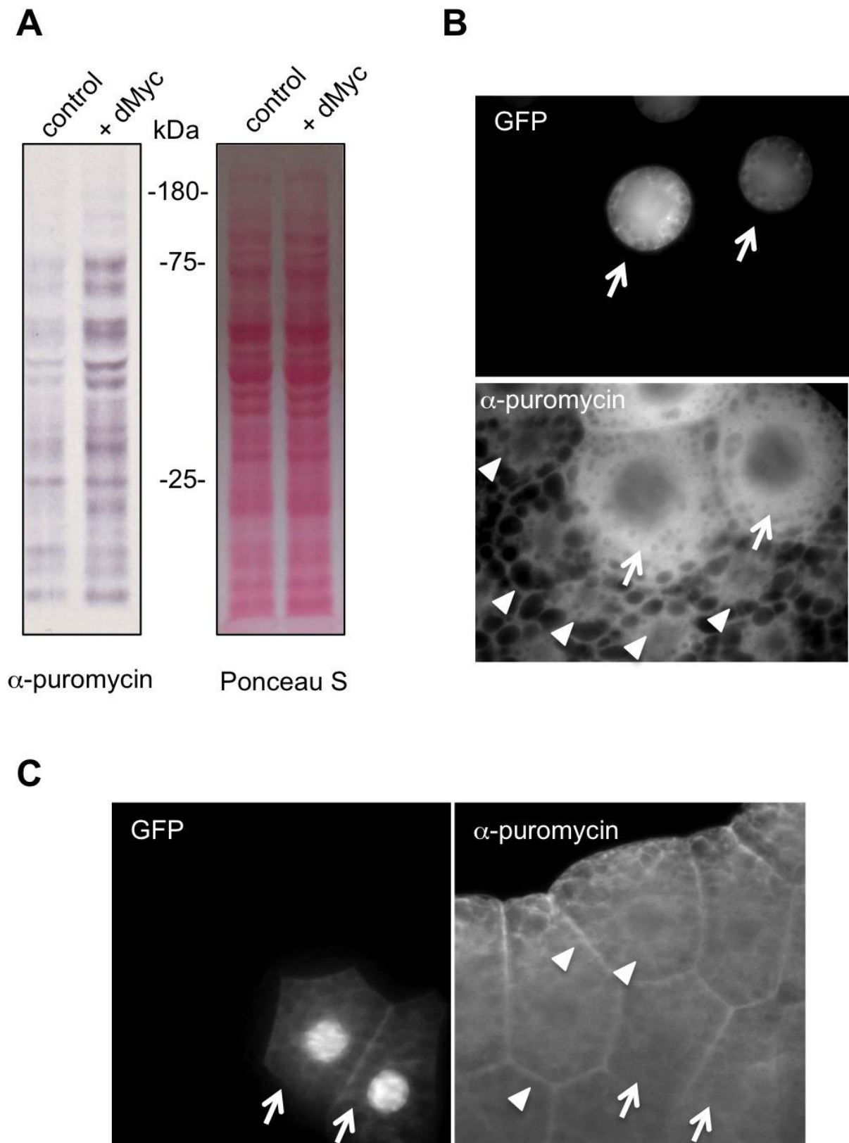
Fig. 3. Regulation of larval protein synthesis by dMyc. (A) The hsflp-out system was used to induce ubiquitous UAS-dMyc expression in third instar larvae. Control larvae expressed UAS-GFP alone. 24hrs following transgene induction. Larvae were inverted and
