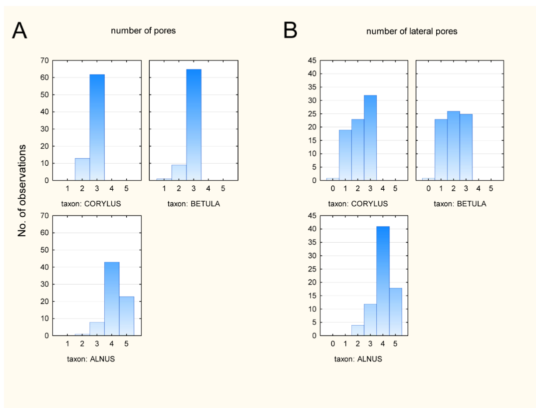
Figure 3. Histograms of A) the number of pores and B) the number of lateral pores for the studied taxa. The sample size is equal to 75 observations for each taxa.
