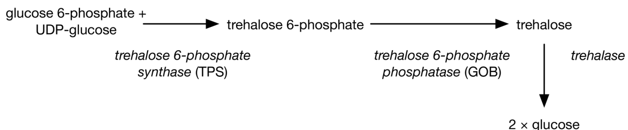
Fig. 3. Schematic outline of trehalose synthesis and degradation in nematodes. Adapted from Behm (1997).
