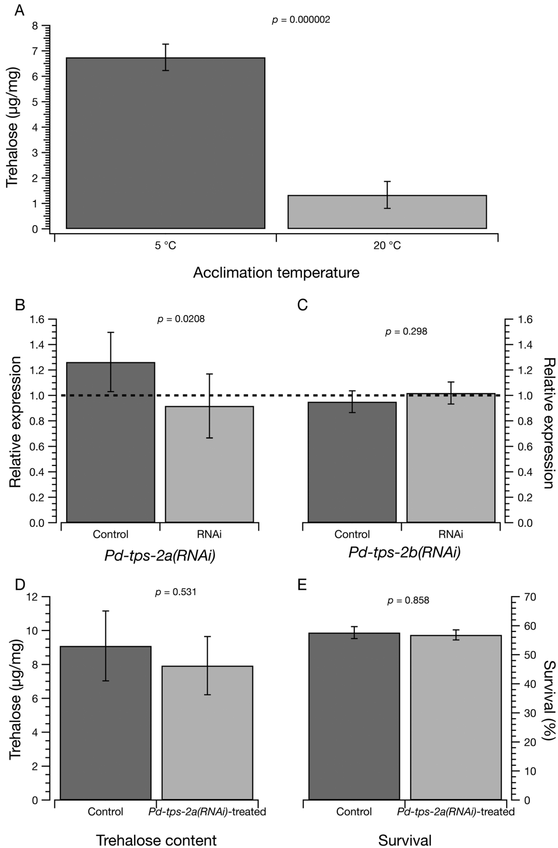
Fig. 2. Analysis of Pd-tps-2a(RNAi) -treated and non-treated (control) samples in response to cold acclimation. (A) Trehalose content of nematodes acclimated at 5°C and 20°C for 72 h was determined by gas chromatography and expressed as \mu\text{g} trehalose/mg of nematode dry weight. (B, C) Gene expression of Pd-tps-2a and Pd-tps-2b after RNAi. Relative expression of each locus is shown as for Fig. 1. (D) Trehalose content of control and RNAi-treated nematodes. (E) Freezing survival of control and RNAi-treated nematodes after freezing at -15^\circ\text{C} for 30 min as described.
